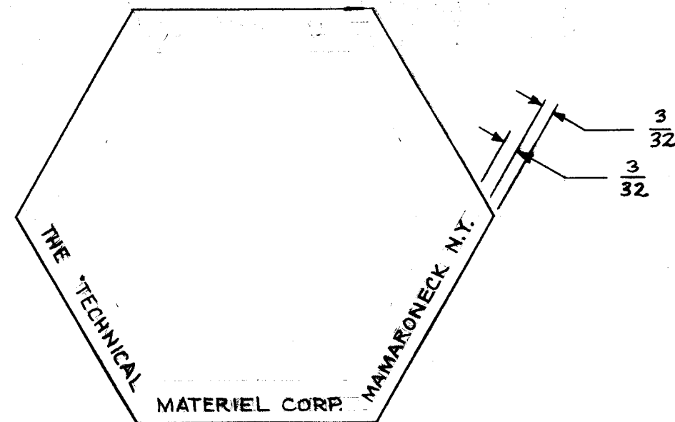
STAMPING DETAIL ITEM 10
