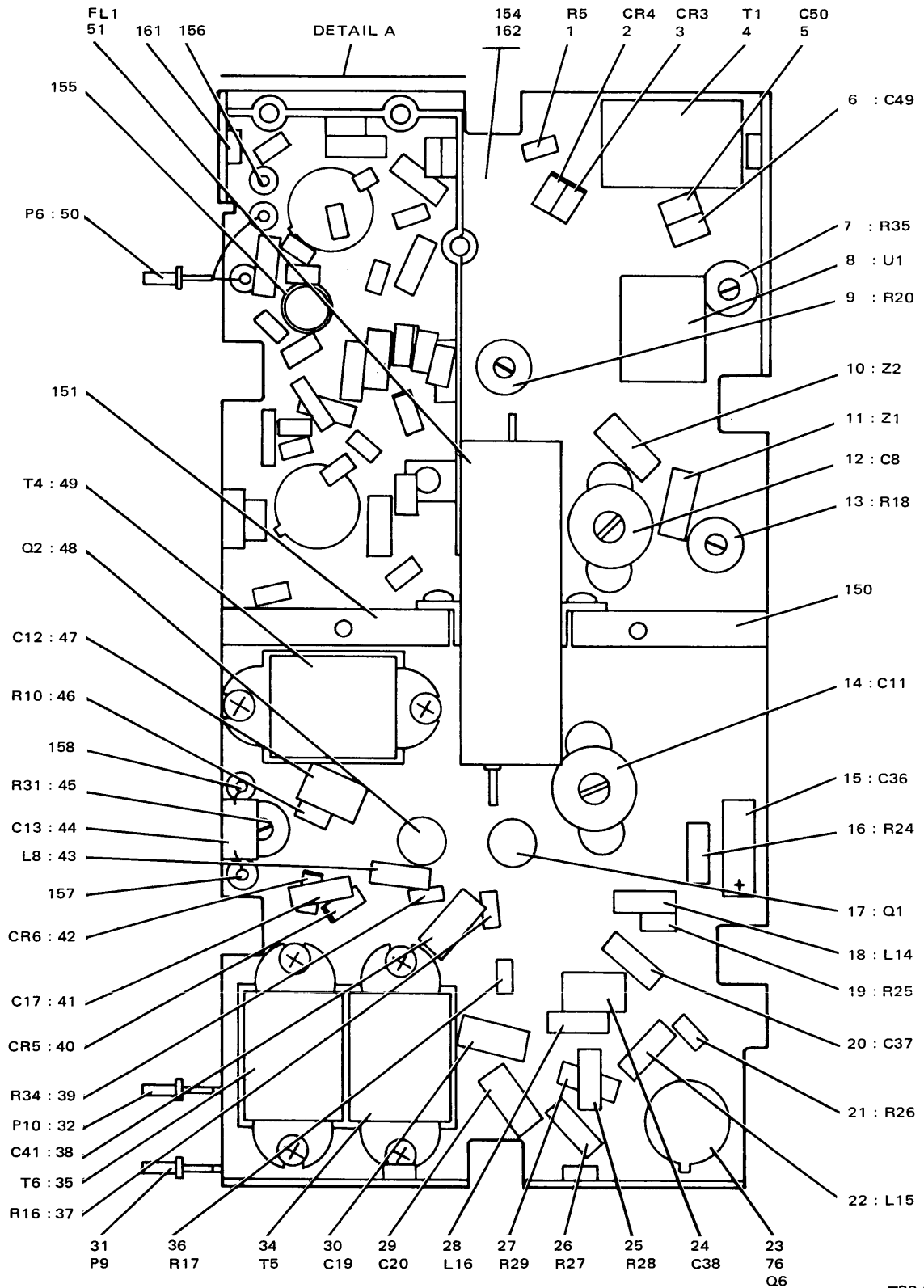
Radio Frequency Mixer (A6A1) 618-3258-001 Figure 37 (Sheet 1 of 3)
