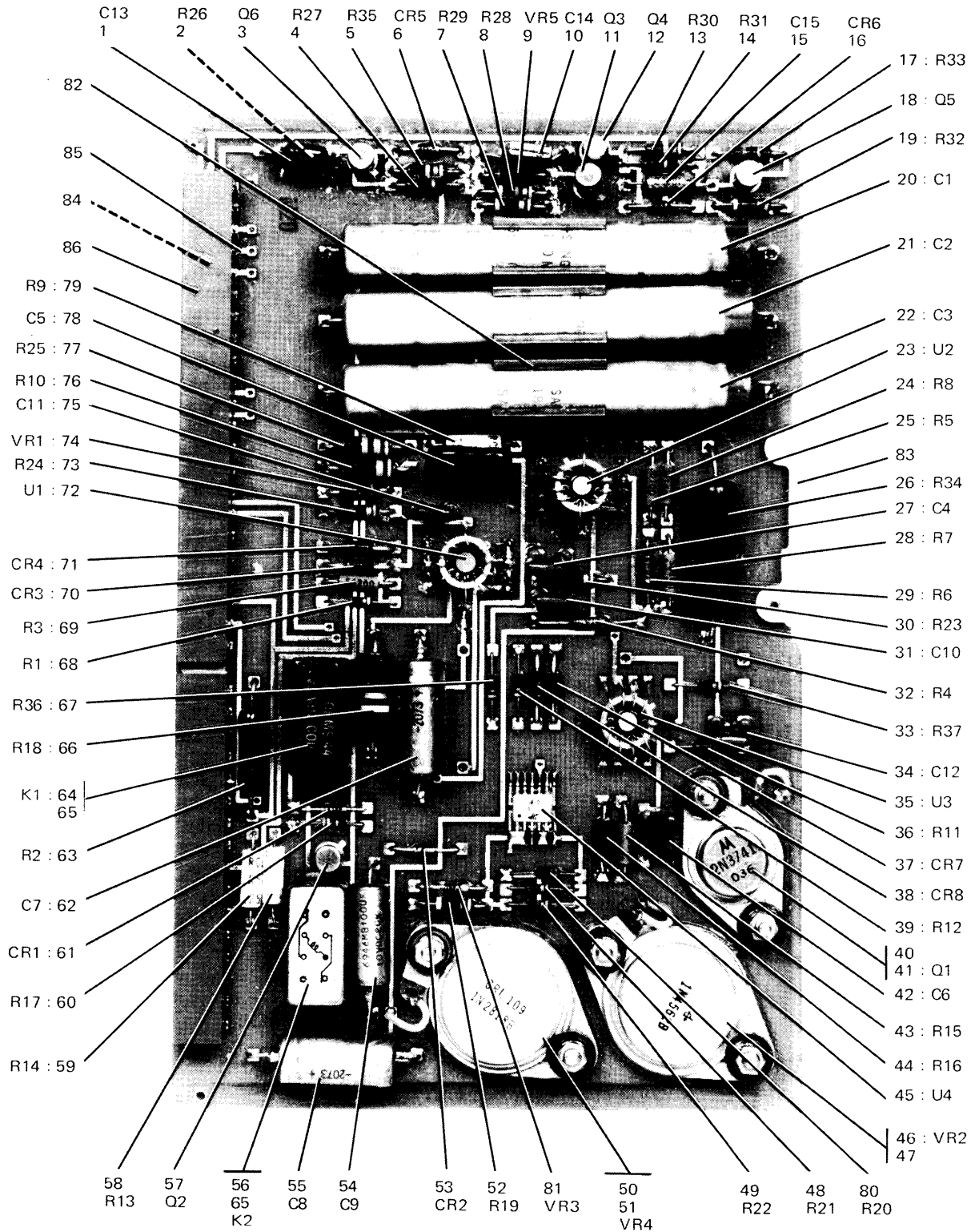
Power Supply Regulator Circuit Card Assembly (A1) 778-2949-001 Figure 24
