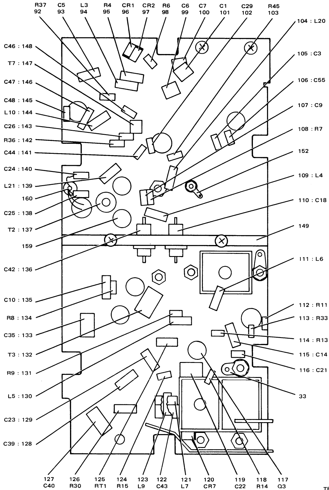
Radio Frequency Mixer (A6A1) 618-3258-001 Figure 37 (Sheet 3 of 3)
