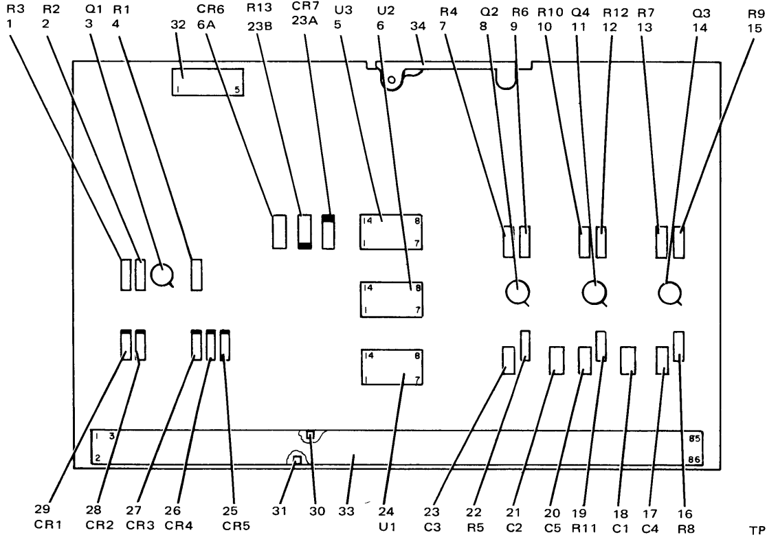
Decoder/Driver Circuit Card Assembly (A7) 608-9087-001 Figure 34
