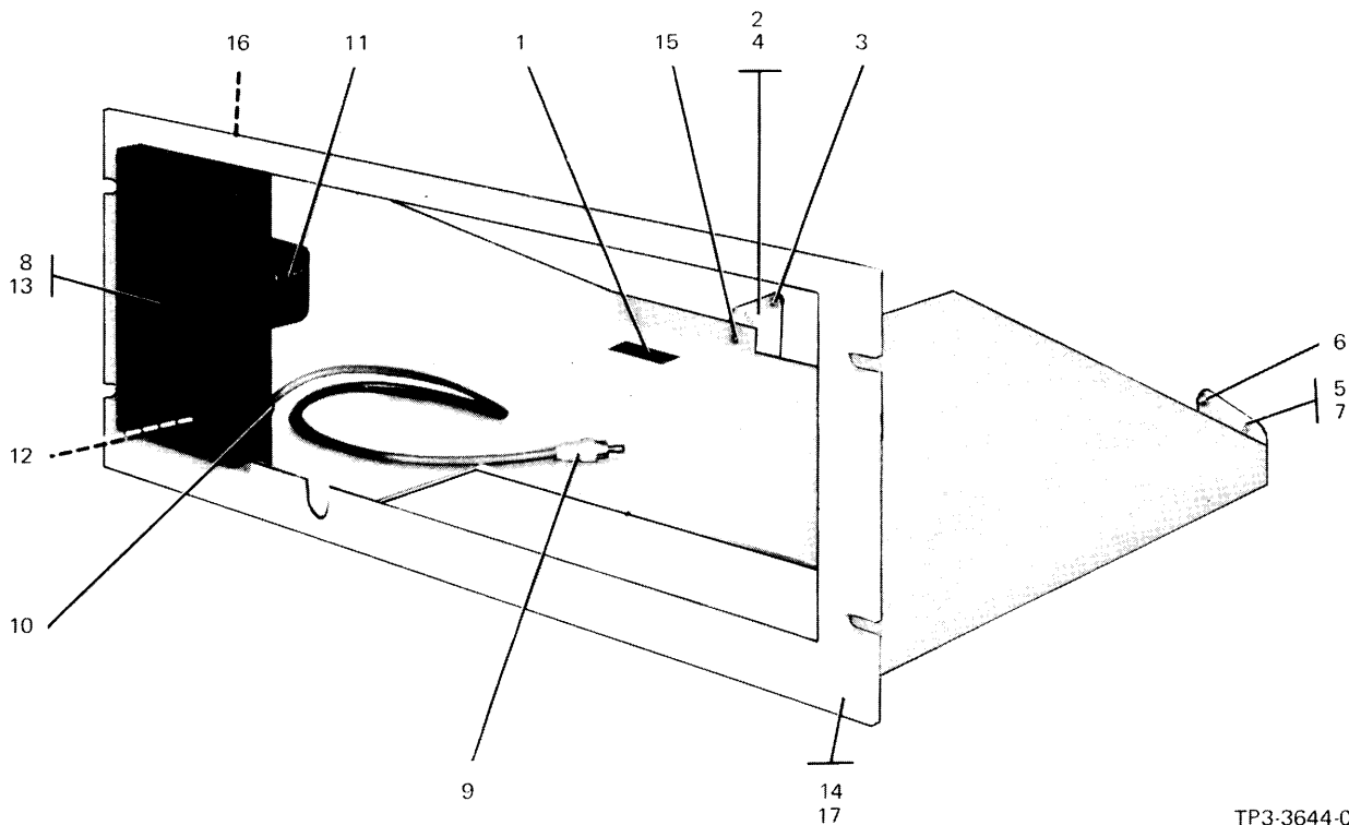
699J-1 Receiver Adapter Figure 42
