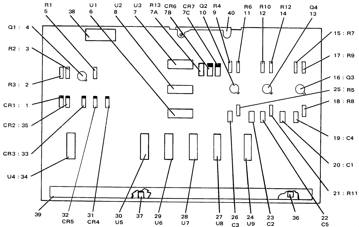
Decoder/Driver Circuit Card Assembly (A7) 608-9121-001 Figure 35
