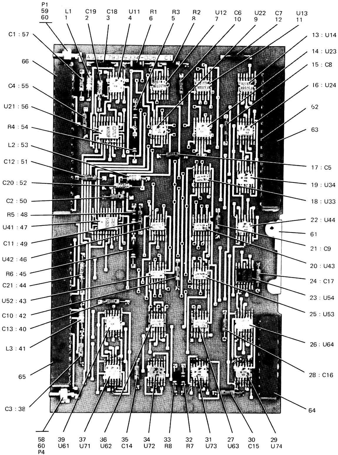
Synthesizer Divider Circuit Card Assembly (A10) 793-9334-006 Figure 9
