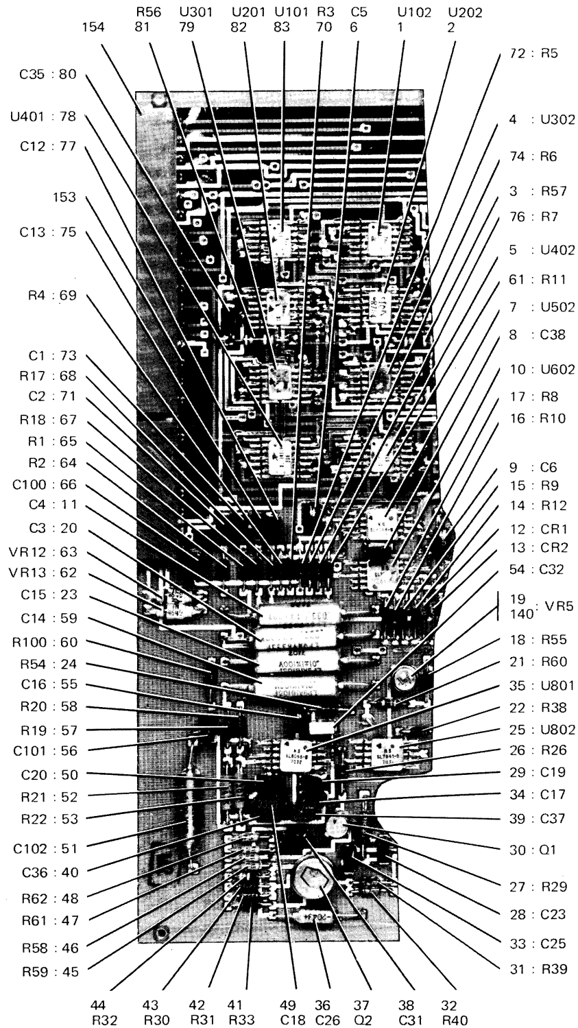
DCU Circuit Card Assembly (A9) 793-9414-001 Figure 11 (Sheet 1 of 2)
