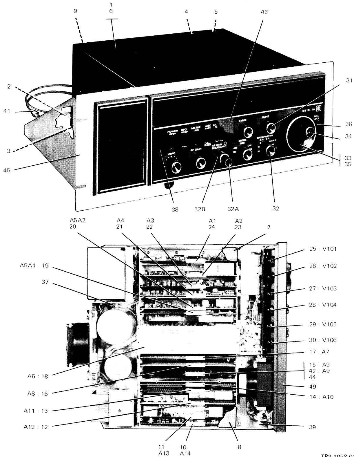
651S-1/1A General Purpose HF Receiver Figure 1
