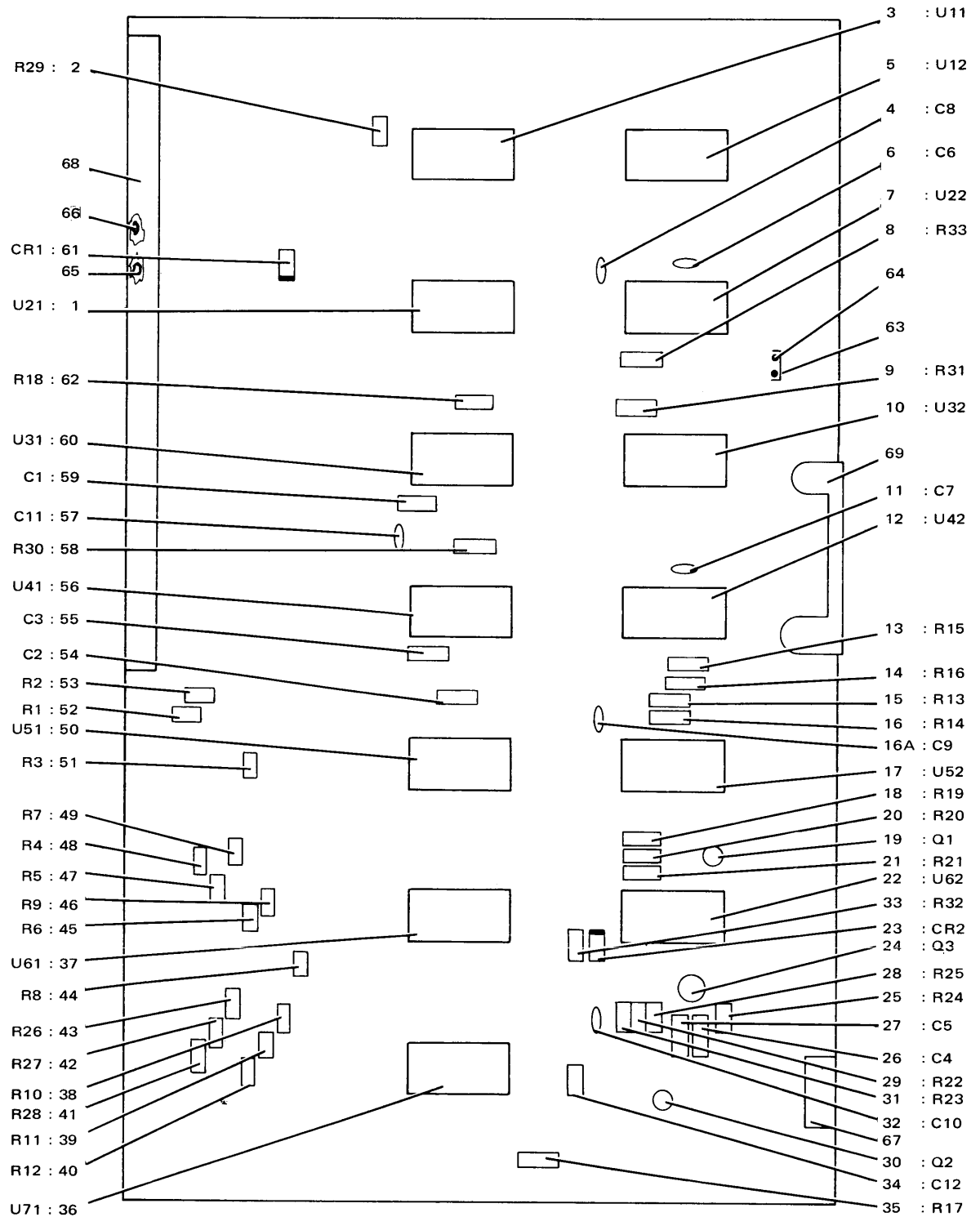
Auto Scan Control Circuit Card Assembly 783-9368-001 Figure 41
