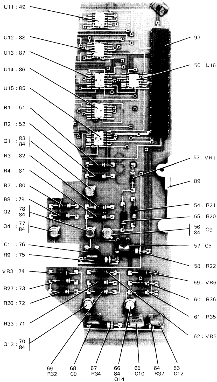
Decoder/Driver Circuit Card Assembly (A7) 778-2928-003 Figure 15 (Sheet 2 of 2)
