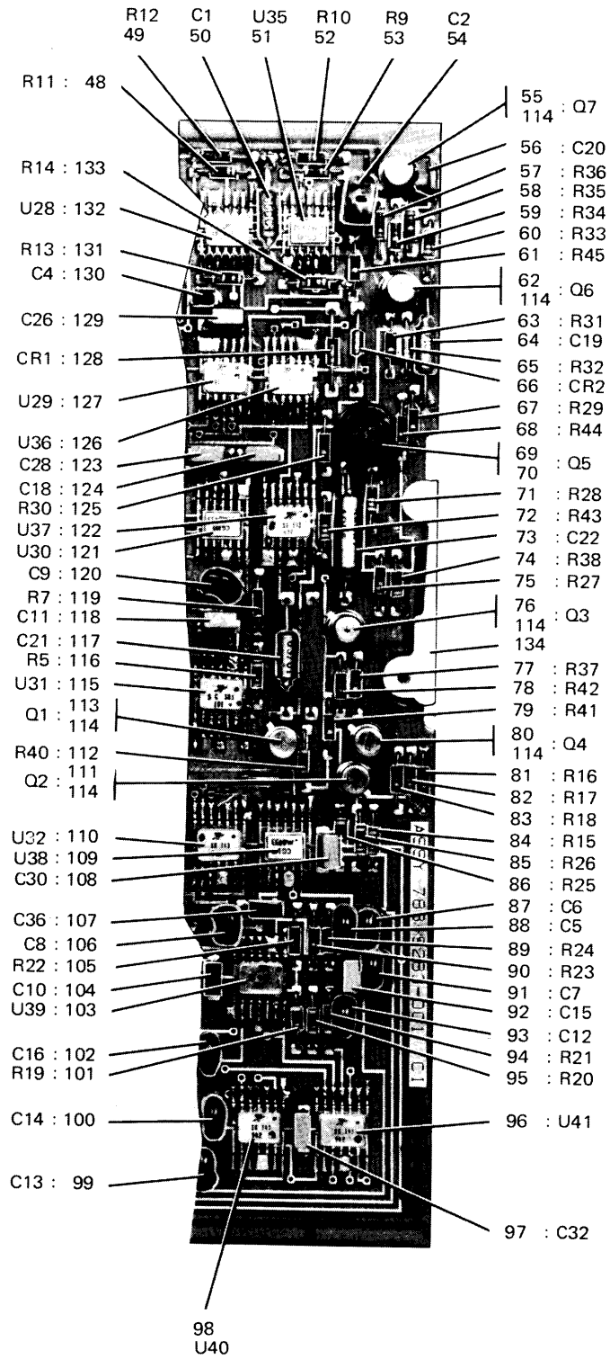
Frequency Control Circuit Card Assembly (A14) 783-9283-001 Figure 2 (Sheet 2 of 2)
