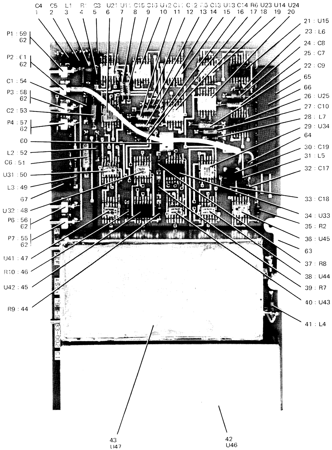
Synthesizer Reference Circuit Card Assembly (A11) 793-9333-002 Figure 6
