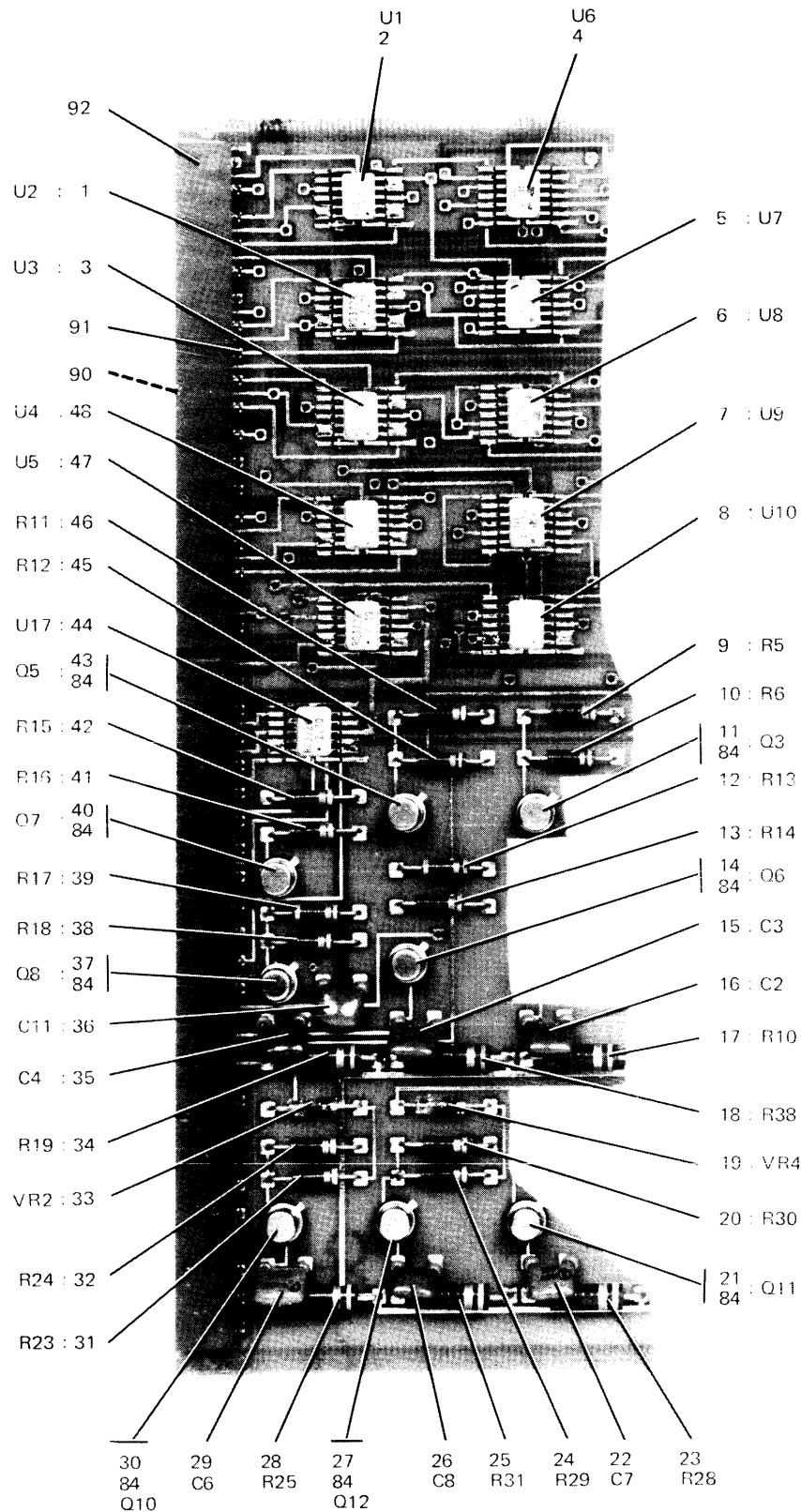
Decoder/Driver Circuit Card Assembly (A7) 778-2928-003 Figure 15 (Sheet 1 of 2)
