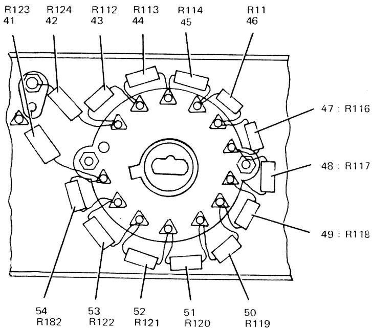
Front Panel Assembly 606-9425-003, -004, -005 Figure 39 (Sheet 2 of 3)
