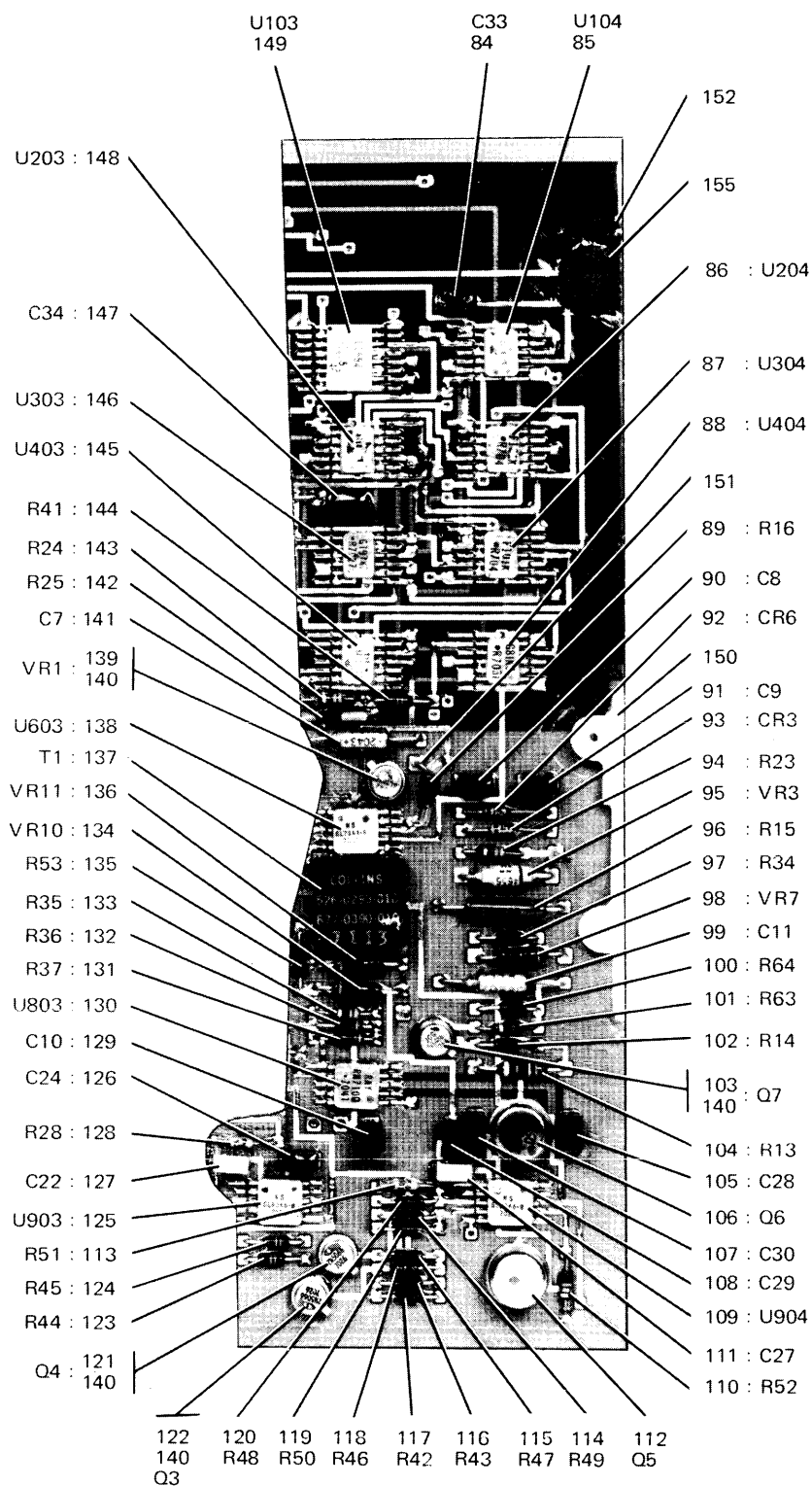
DCU Circuit Card Assembly (A9) 793-9414-001 Figure 11 (Sheet 2 of 2)
