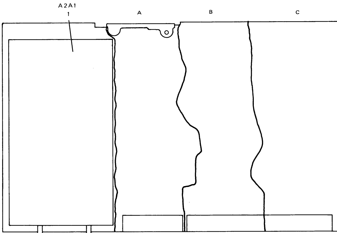
Audio Amplifier Circuit Card Assembly (A2) 778-2948-002, -004 Figure 25 (Sheet 1 of 4)
