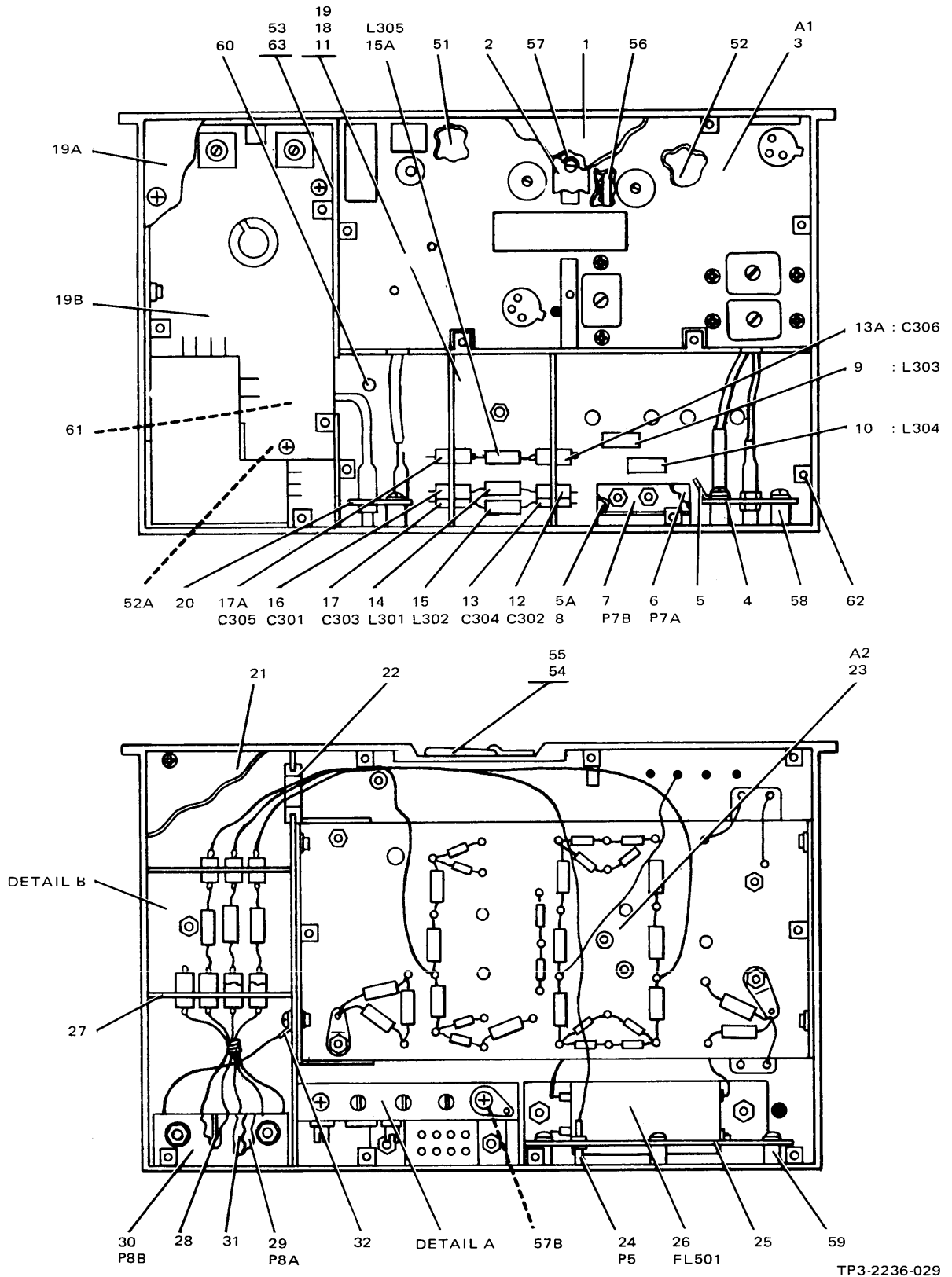
RF Module Assembly (A6) 790-1048-020, -021 Figure 36 (Sheet 1 of 2)
