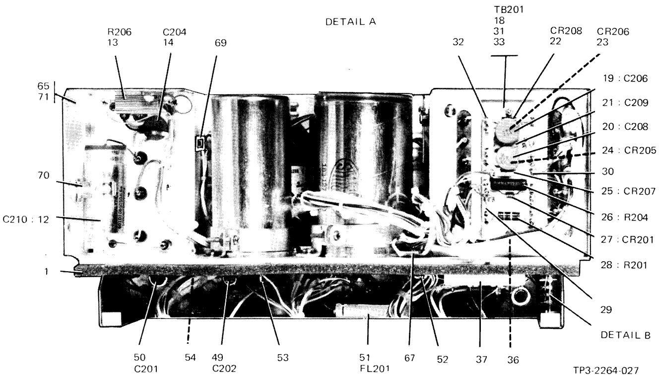
Radio Receiver Power Supply 606-9424-002, -004, -005, -006 Figure 40 (Sheet 1 of 2)
